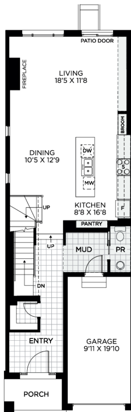
GROUND FLOOR
