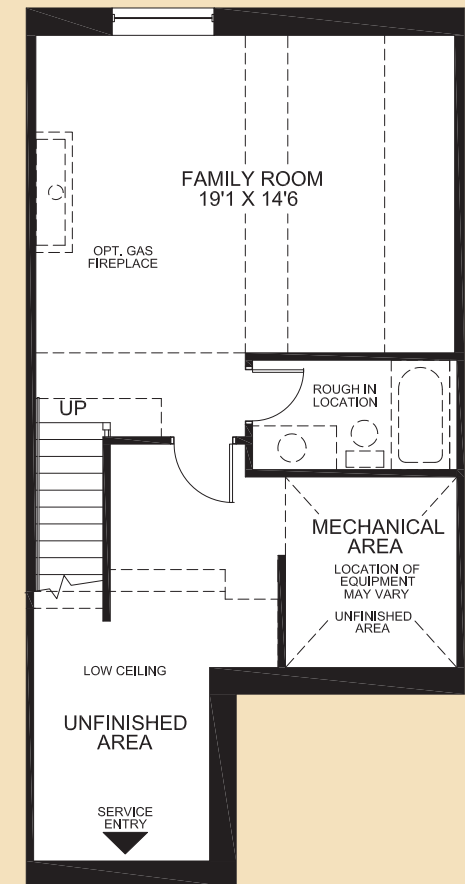
BASEMENT FINISHED AREA 349 Sq. Ft.
