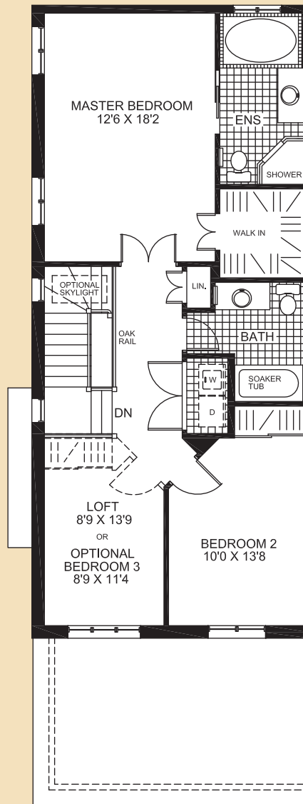
BEDROOM FLOOR 3 BEDROOM OR 2 WITH LOFT & LUXURY ENSUITE
