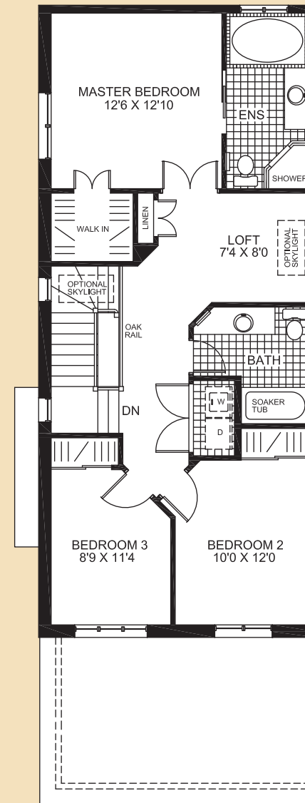
OPTIONAL BEDROOM FLOOR 3 BEDROOM WITH LOFT & LUXURY ENSUITE
