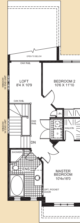
OPTIONAL BEDROOM FLOOR 2 BEDROOM WITH LOFT & LUXURY BATH
