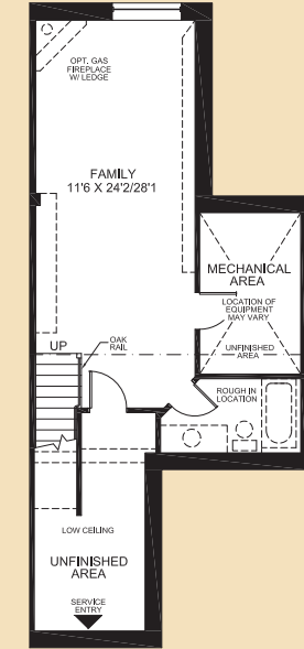
BASEMENT FINISHED AREA 353 Sq. Ft.
