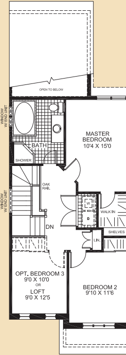
OPTIONAL BEDROOM FLOOR 3 BEDROOM OR 2 WITH LOFT & LUXURY BATH
